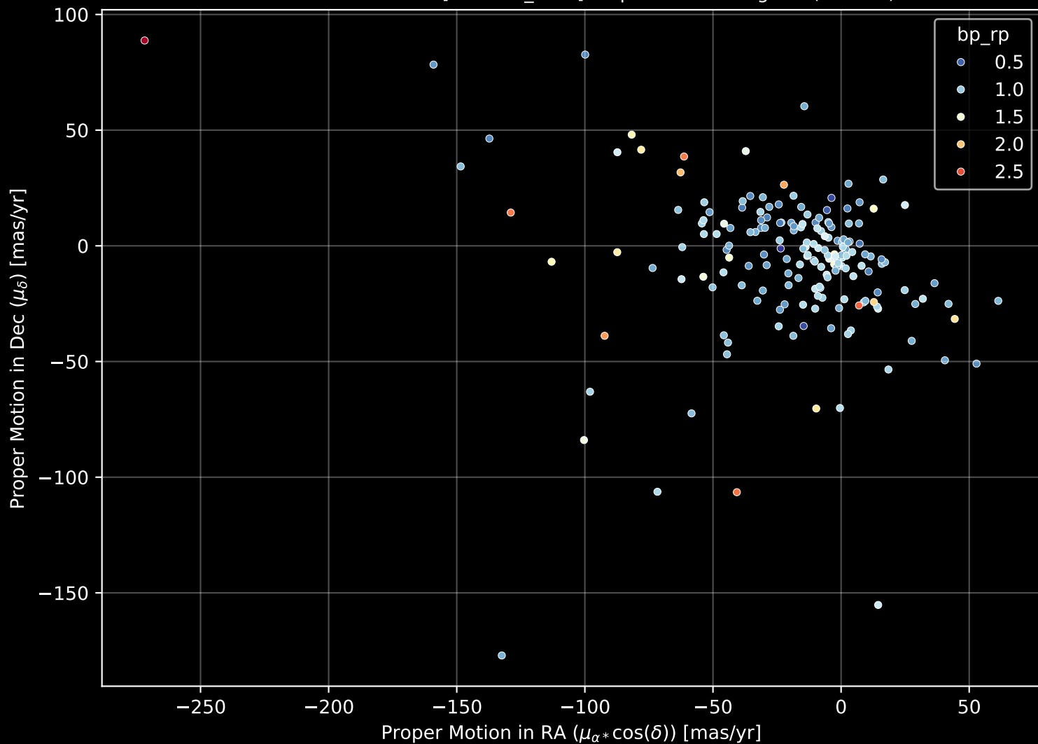
APOGEE DR17 Field: [016+77_MGA] Proper Motion Diagram (n= 184)
