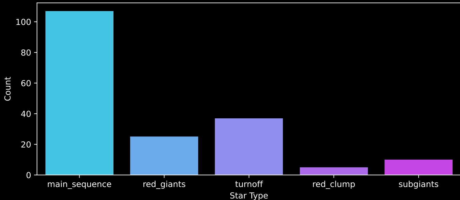
APOGEE DR17 Field: [016+77_MGA] Count plot of Star Type
