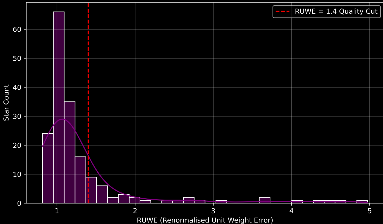
GAPOGEE DR17 Field [016+77_MGA] RUWE Distribution (n= 177)
