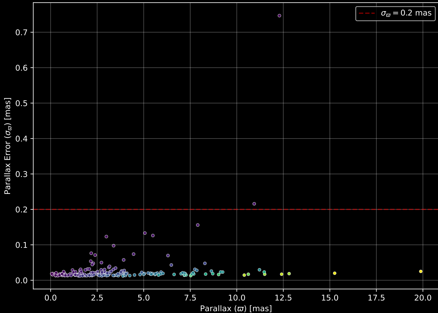
APOGEE DR17 Field: [016+77_MGA] Parallax Quality (n= 184)
