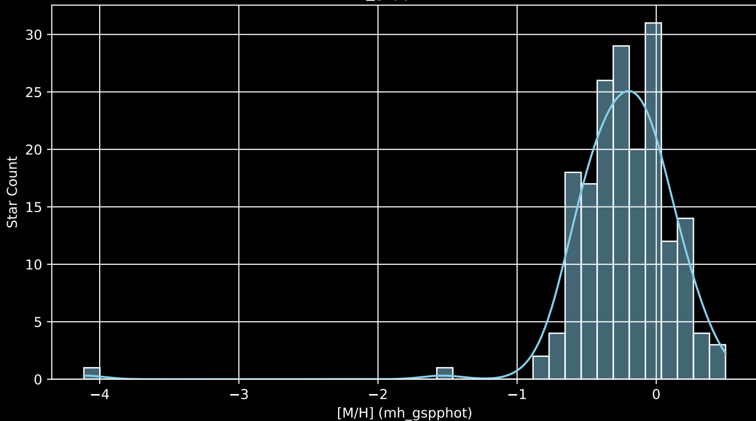
APOGEE DR17 Field: [016+77_MGA [M/H] (mh_gspphot) (n= 182)
