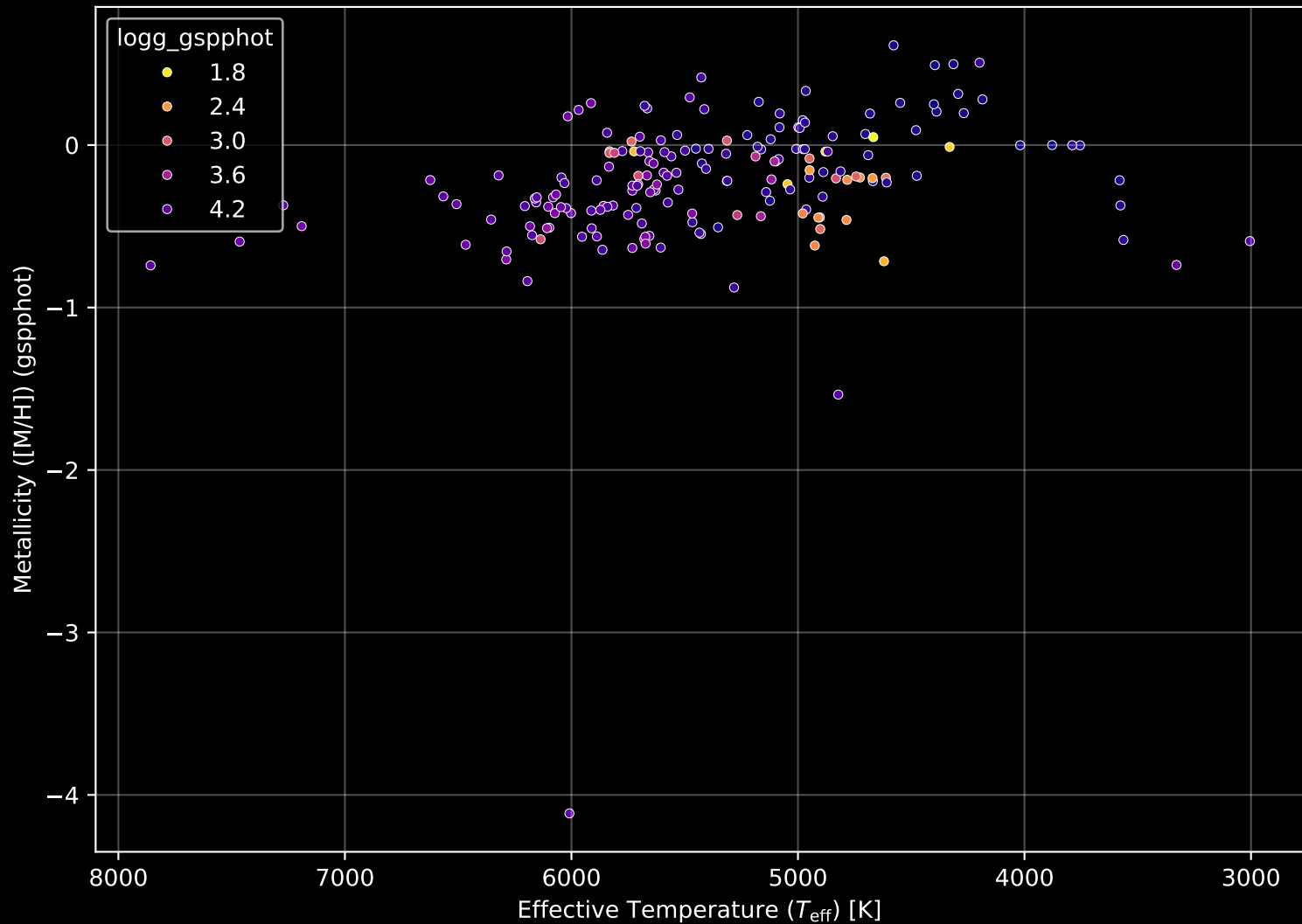
APOGEE DR17 Field: [016+77_MGA] Stellar Population Parameters (n= 184)
